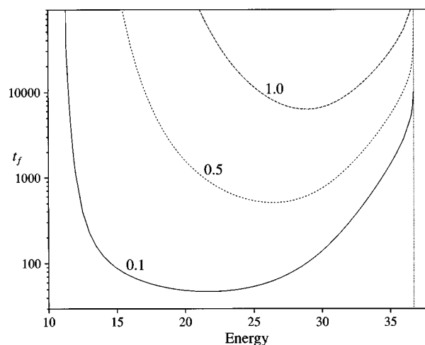
FIG. 7. The dependence of t_f on the barrier height b for our standard PES. t_f is defined by P_1(t_f)=0.8 . The vertical dotted line denotes the energy at which P_1^{\text{eq}}=0.8 . Each line is marked by the value of b .
