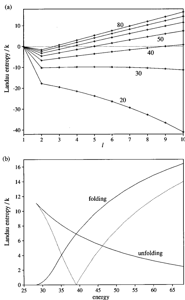
FIG. 4. (a) Landau entropy profiles for our standard PES using the order parameter l . The seven lines shown are for E = 20 - 80 in intervals of 10 and are labeled by the appropriate value of E . (b) Depth of the Landau entropy bottleneck relative to the Landau entropy maximum at large values of l (“folding”) and relative to the Landau entropy maximum at the global minimum (“unfolding”). The dashed line gives the magnitude of the Landau entropy difference between the two stable states.
