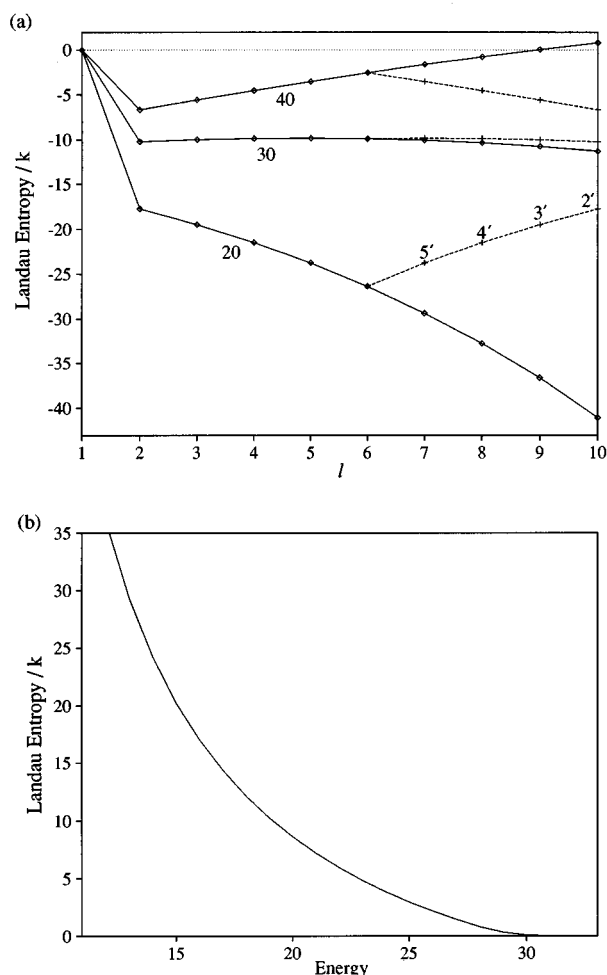
FIG. 11. (a) Landau entropy profiles for a PES with two funnels and l_{\text{node}}=6 . The lines are labeled by the corresponding values of the energy. The dashed lines are for the secondary funnel and points have been marked by the appropriate value of l' . (b) The energy dependence of the magnitude of the Landau entropy bottleneck for passage from the bottom of the secondary funnel to the primary funnel.
